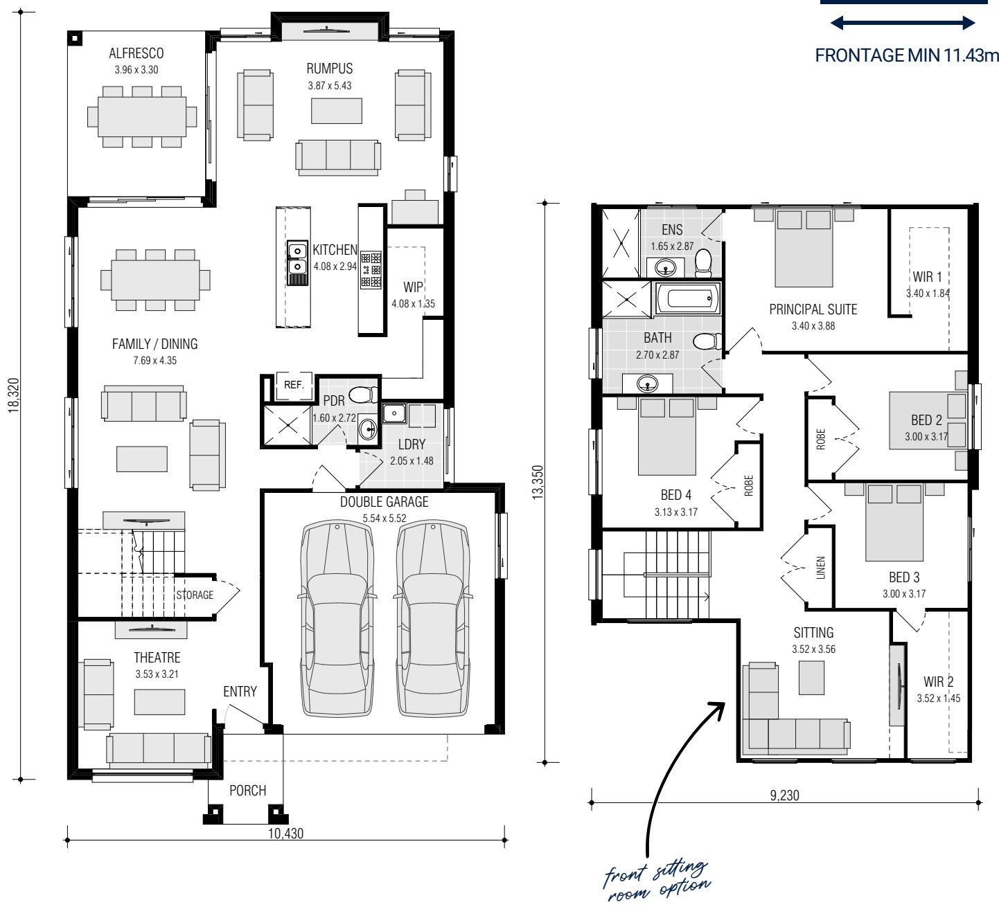
Ground Floor
