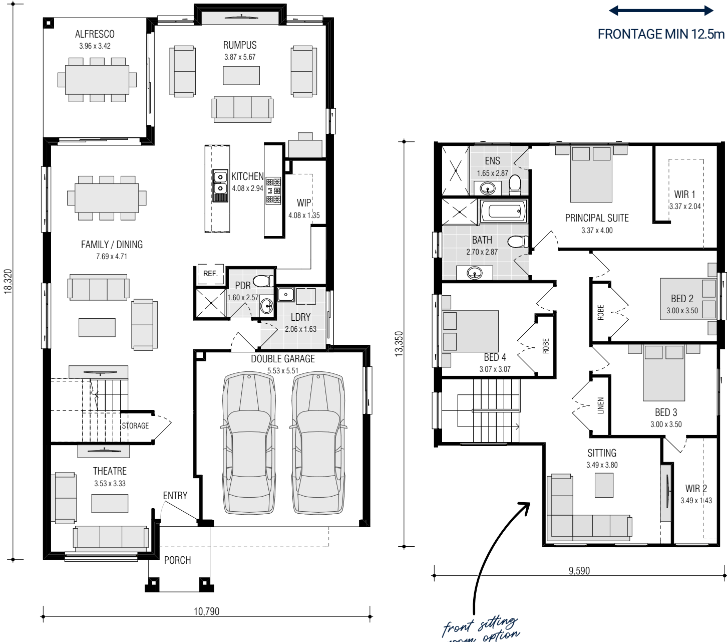
Ground Floor
