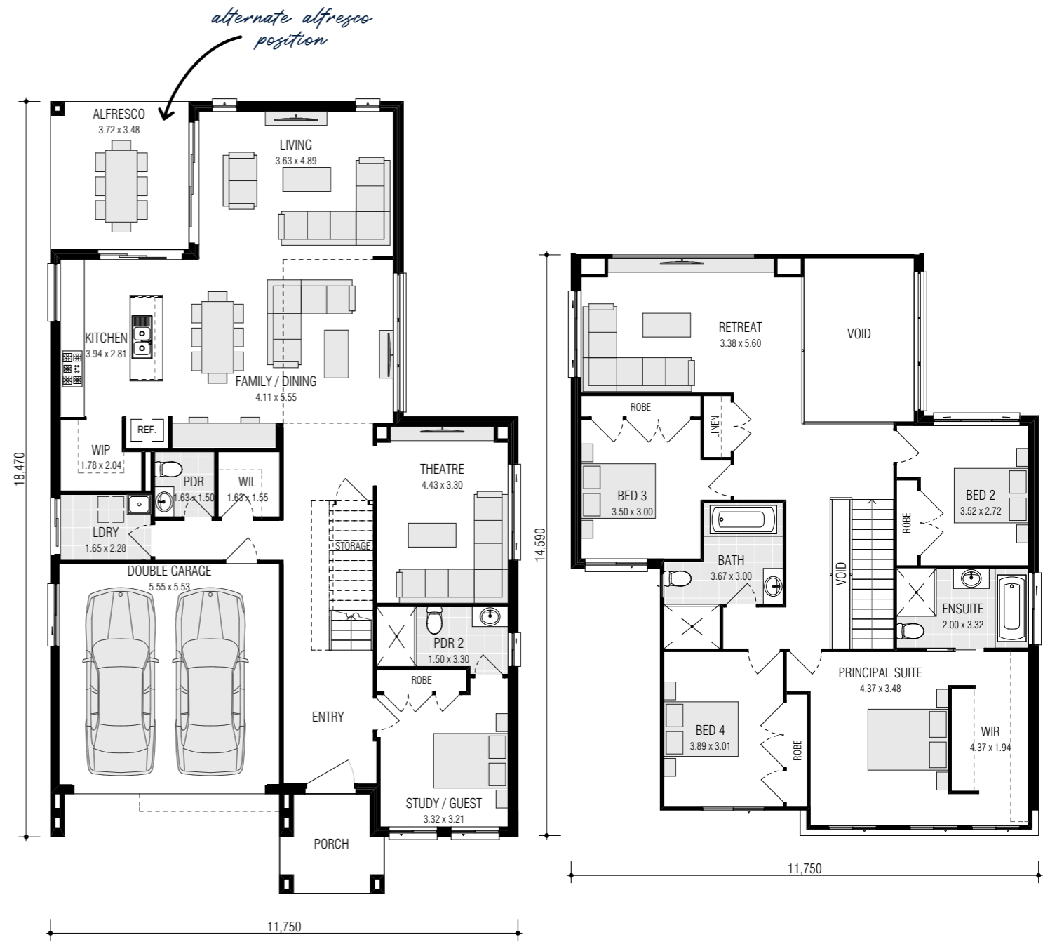
Ground Floor
