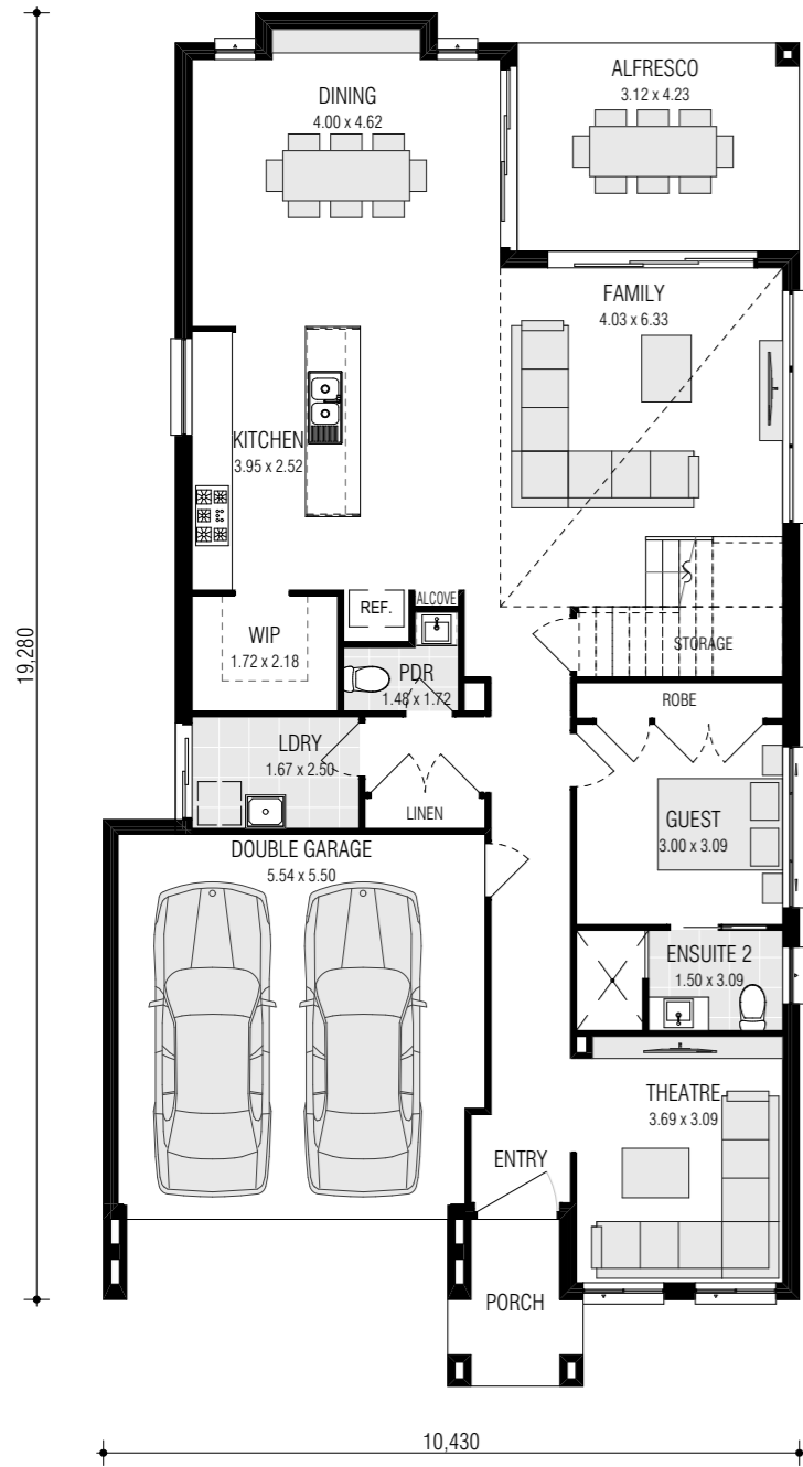
Ground Floor
