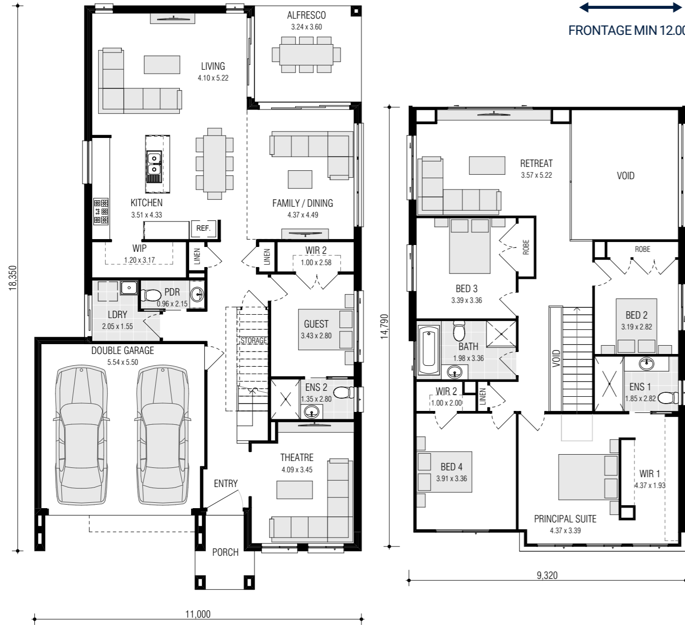
Ground Floor
