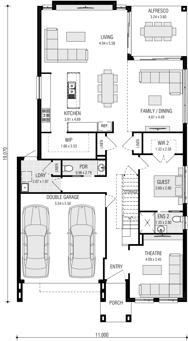
Ground Floor
