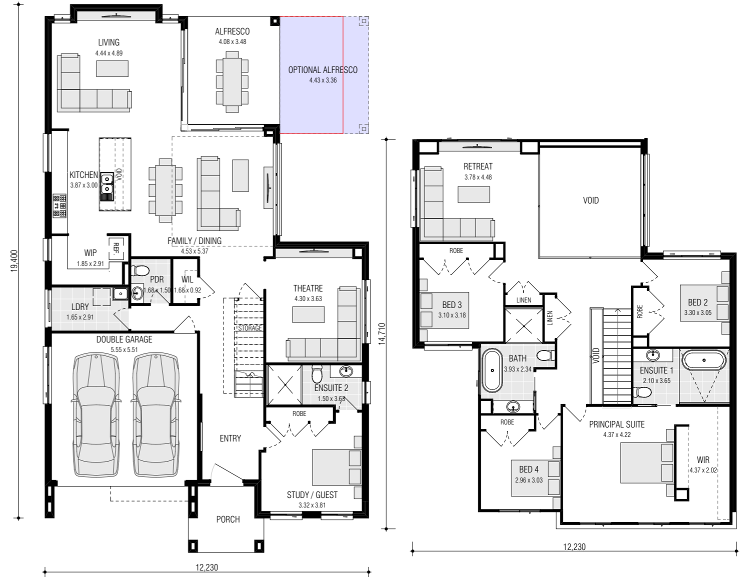
Ground Floor
