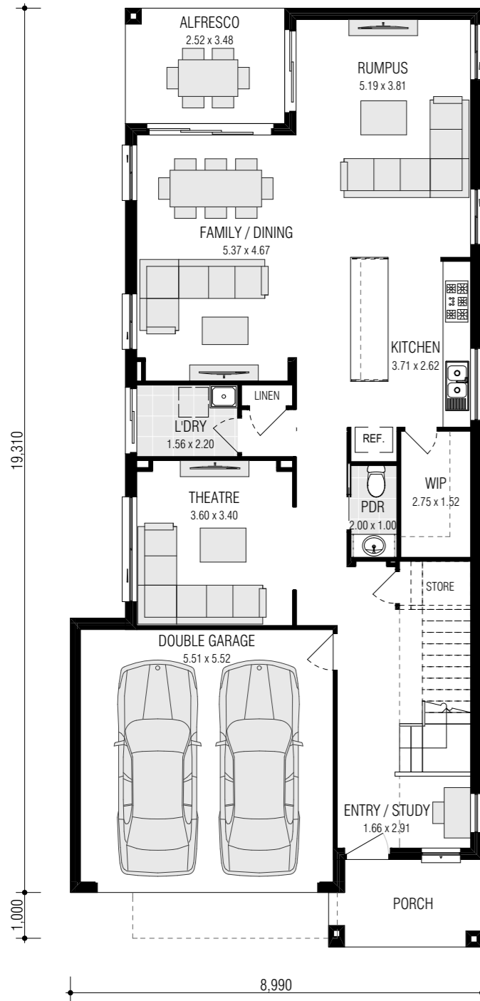
Ground Floor
