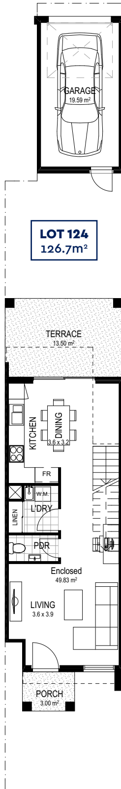
GROUND FLOOR
